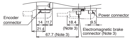
When the cables are led out in opposite direction of load side
