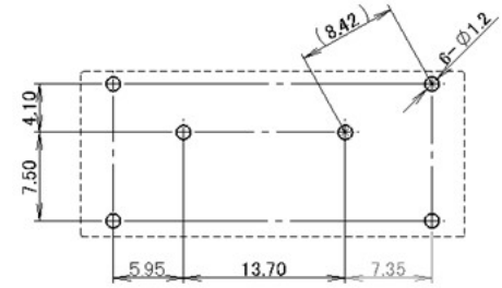
PC-BOARD PATTERN(BOTTOM VIEW) (TOLERANCE: \pm 0.1 )
