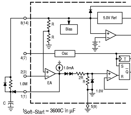
Figure 20. Soft-Start Circuit
