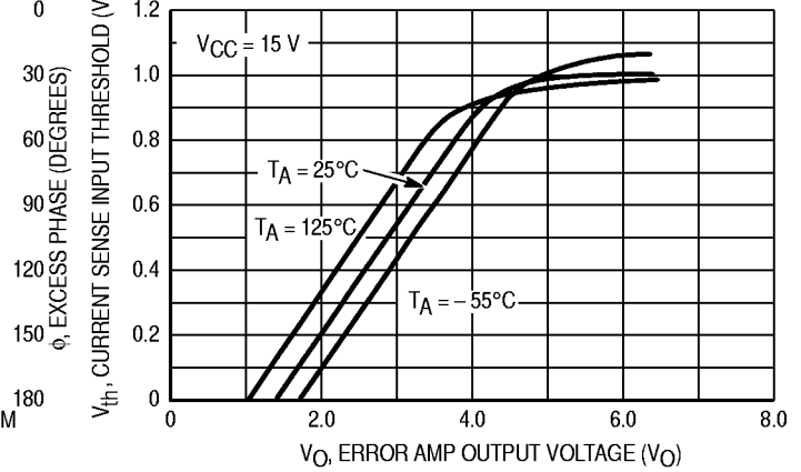
Figure 6. Current Sense Input Threshold versus Error Amp Output Voltage
