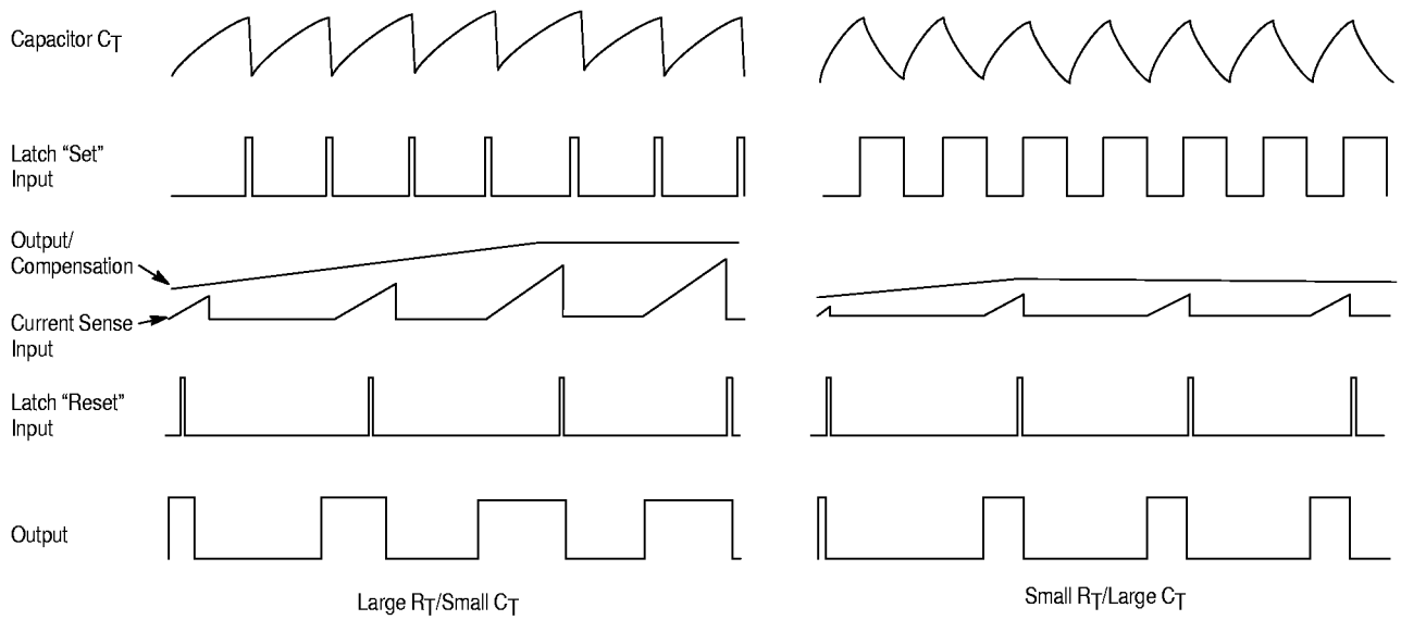
Figure 16. Timing Diagram
