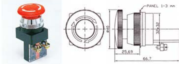
LEPB3011 30φ 急停按鈕
